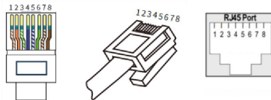
Battery CAN
